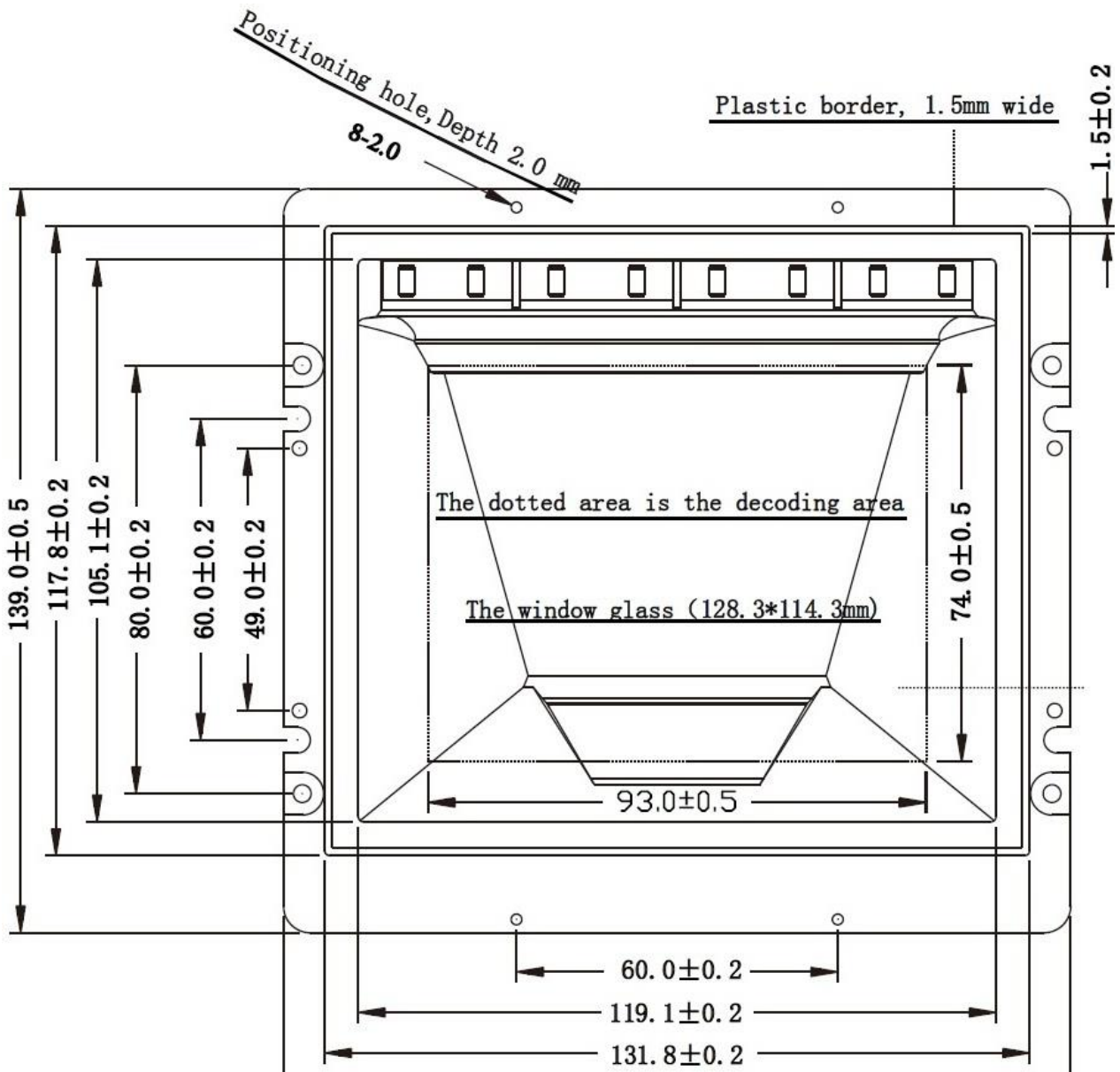
Figure 2-2 Dimensions
